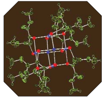
A view of the cube shape showing Pd (blue) and S (red) atoms.
